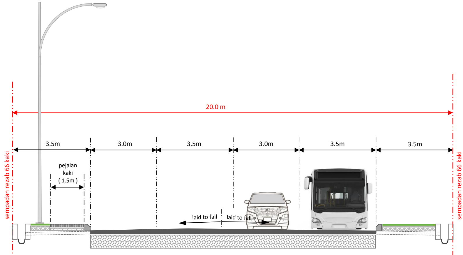
KERATAN 3.50m + 3.0m lebar lorong 1 + 2 lorong @ simpang
